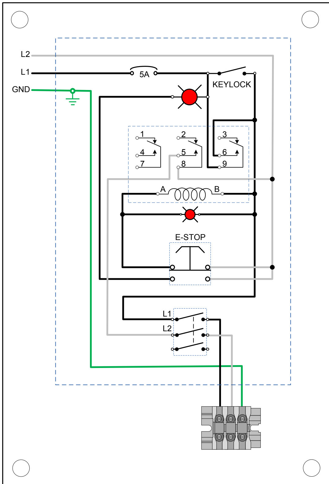
PANEL PC04 120V SINGLE PHASE POWER PANEL Revision A
