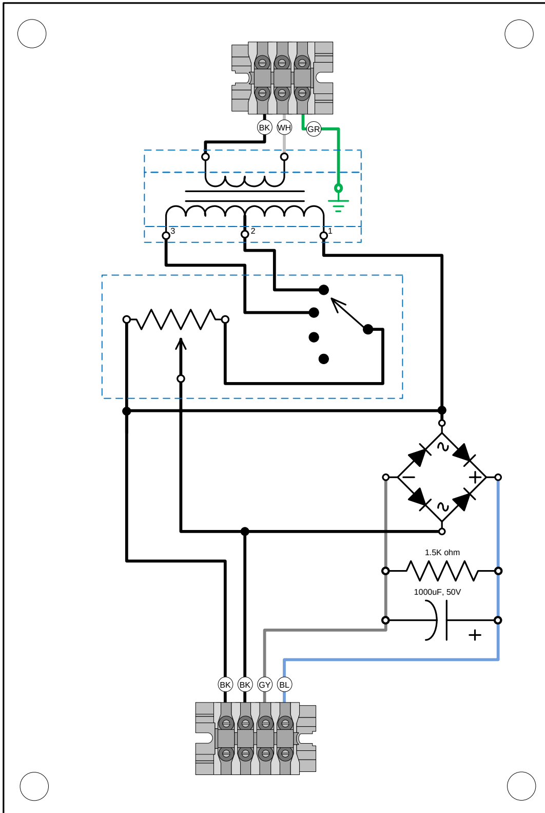
PANEL E152 VARIABLE POWER SUPPLY Revision B
