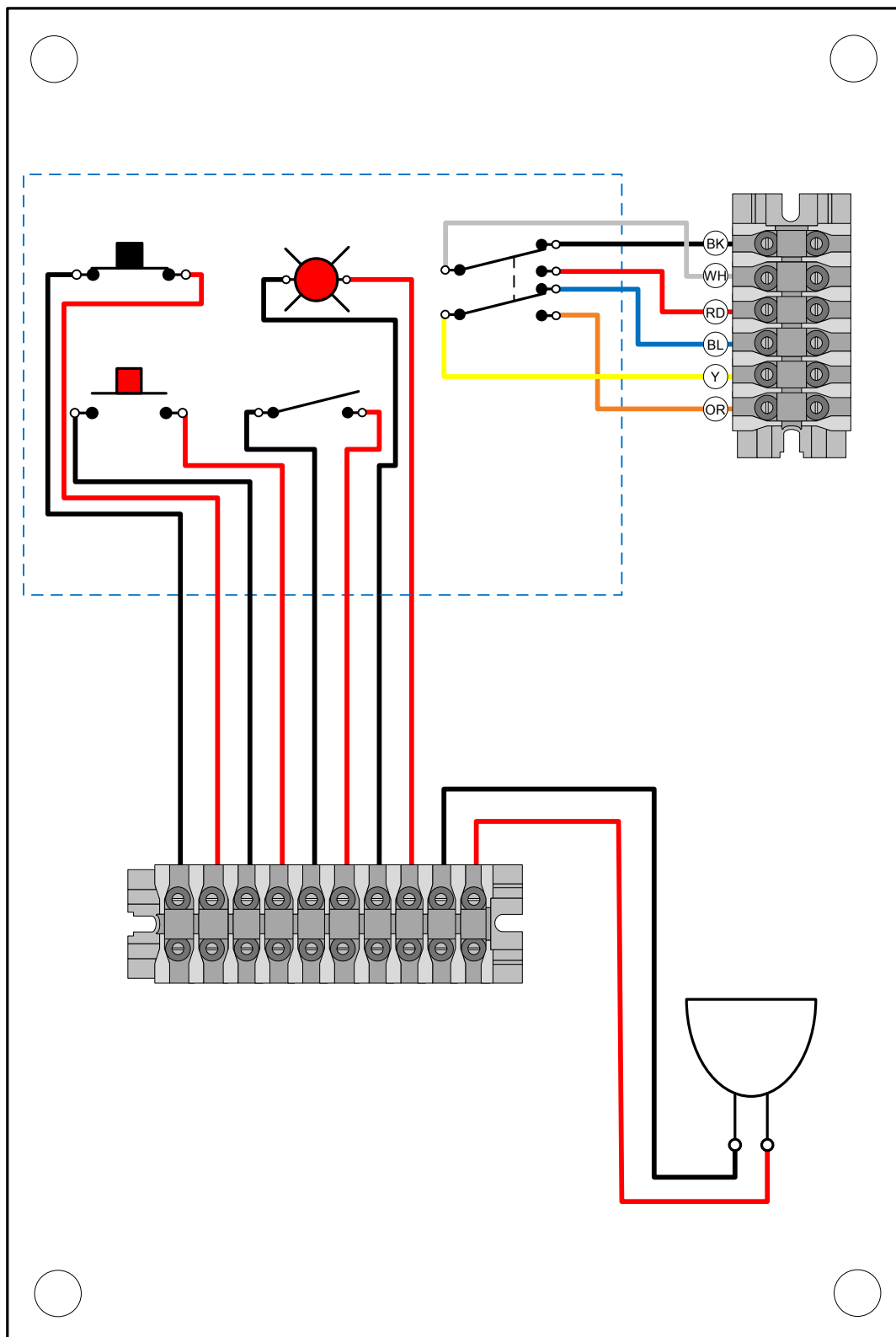
PANEL E040 SWITCH AND LAMP PANEL
